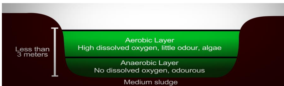
Figure 1: Layering in a facultative pond
