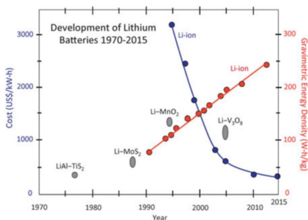
Figure 7.13: Cost reduction in Lithium Batteries (ARENA, 2017)
