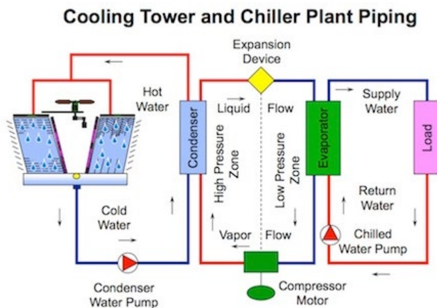
Figure 7.10: Refrigeration circuit with primary and secondary refrigerant (chilled water)
