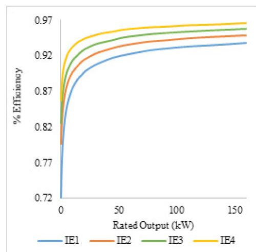
Figure 7.11: IE1 to IE4 bands for 4 pole motors (Carbon Trust, 2018)
